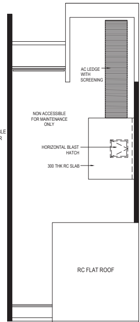
Upper Roof
