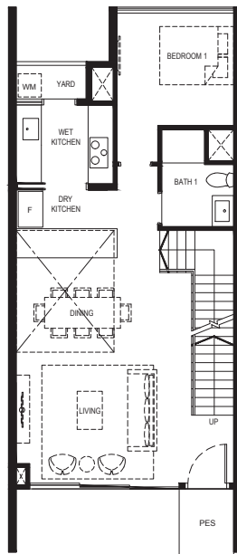
1st Storey
